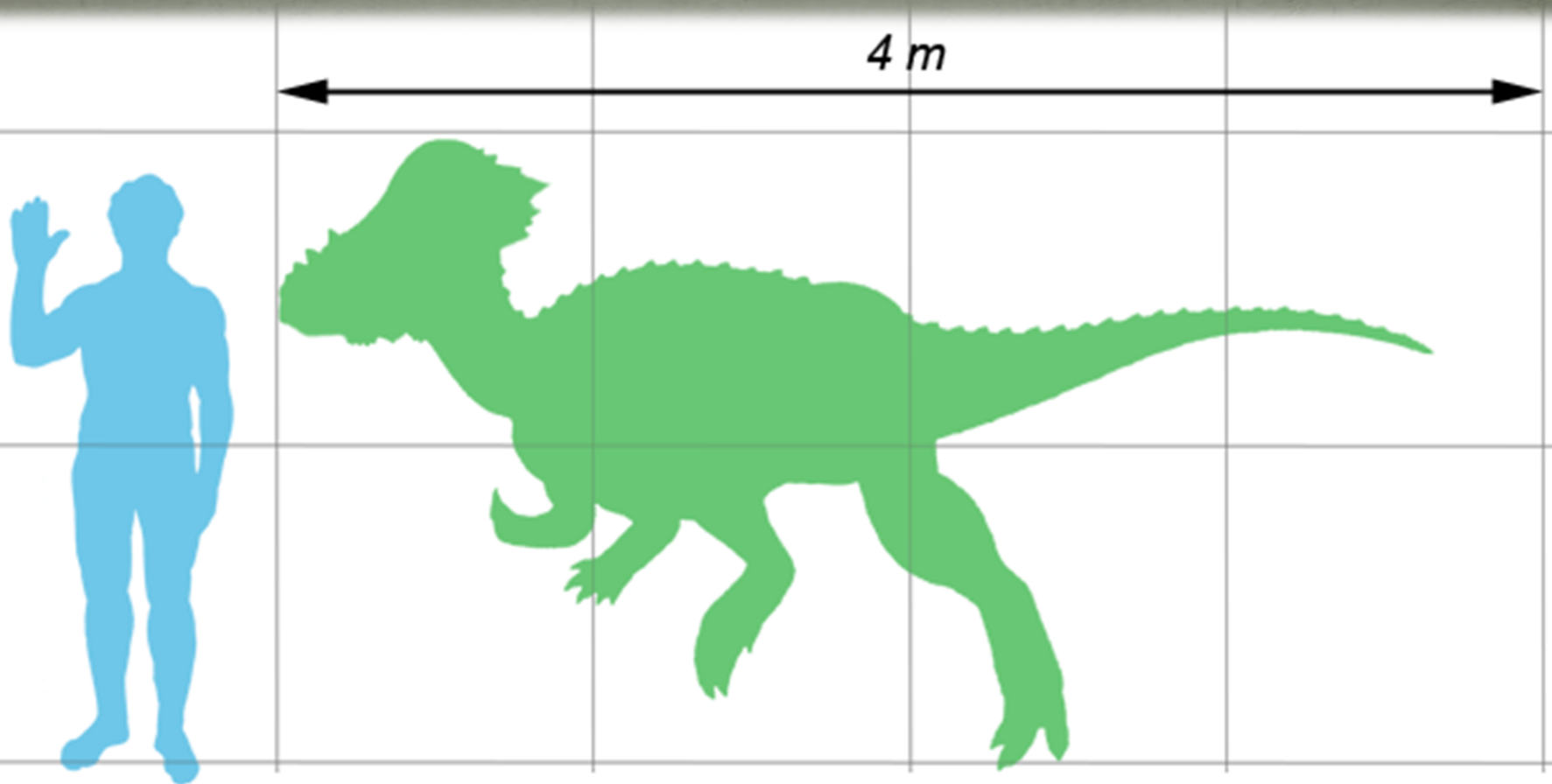
Pachycephalosaurus wyomingensis
